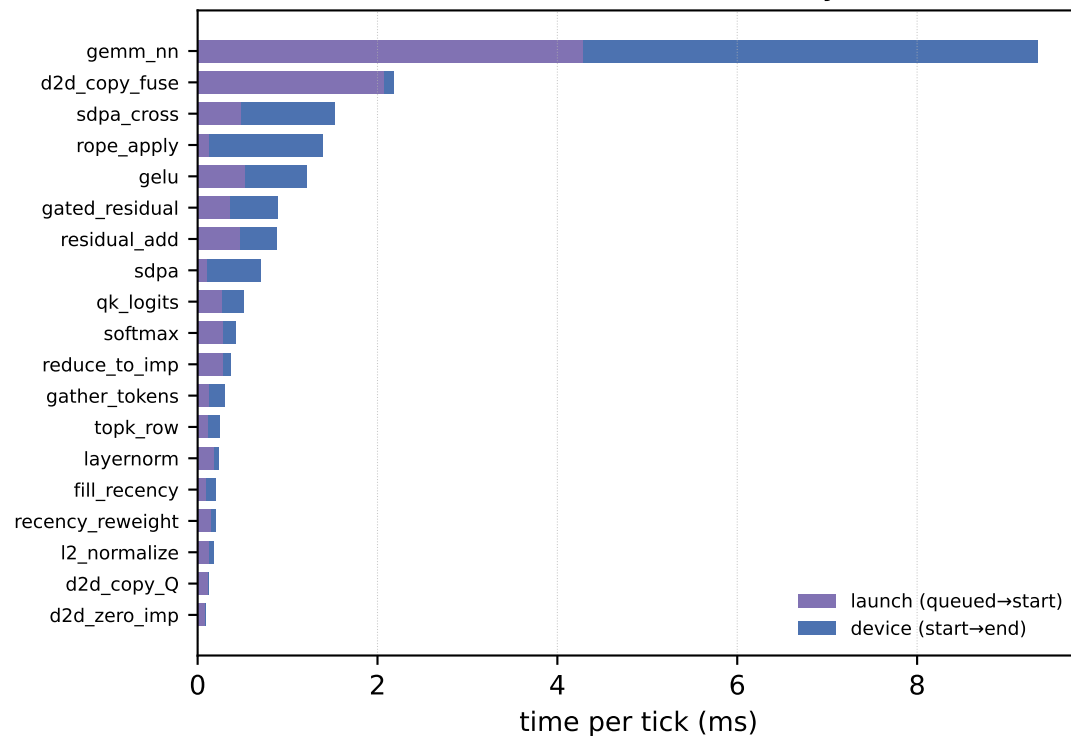
Launch vs device latency
