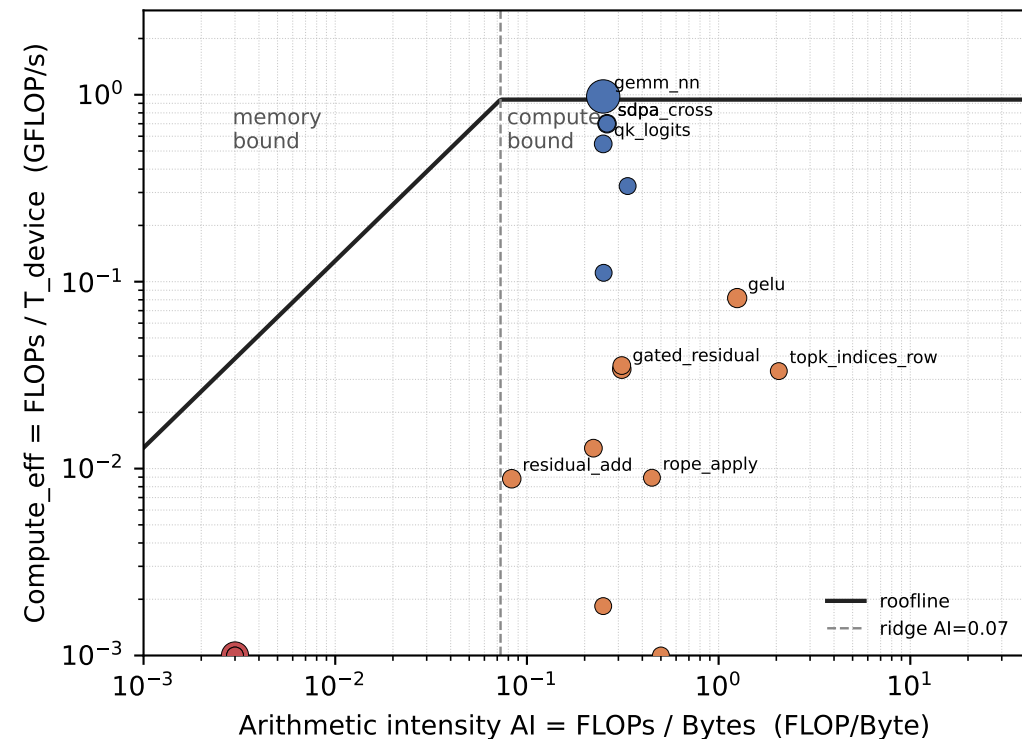
Roofline (device time T)
