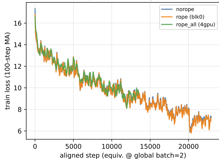
Step loss (batch-aligned)
