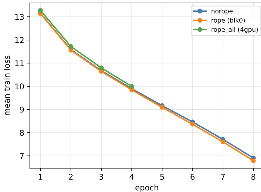
Epoch train loss
