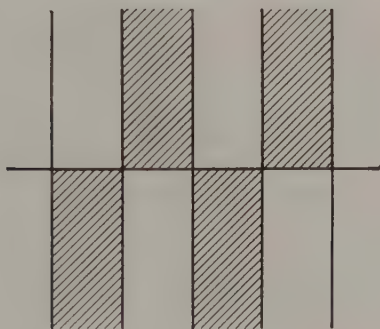
FIG. 3-11. Fundamental regions of \cos z .
