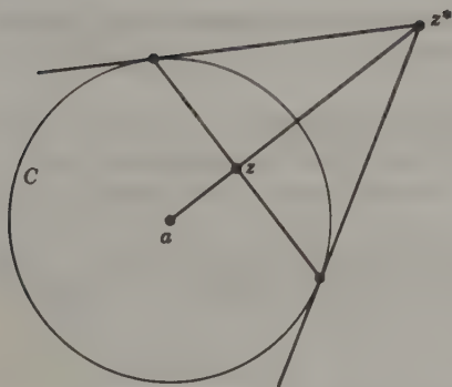
FIG. 3-2. Reflection in a circle.
