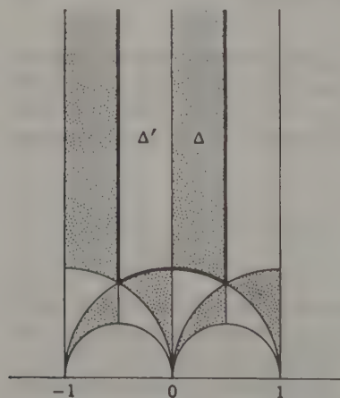
FIG. 7-4. Fundamental region of \lambda(\tau) .
