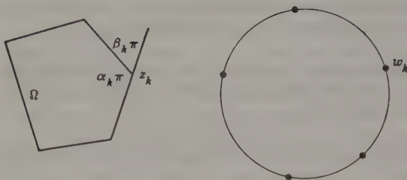
FIG. 6-1. Conformal mapping of a polygon.
