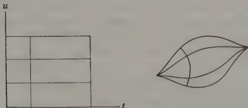
FIG. 8-2. Deformation.
