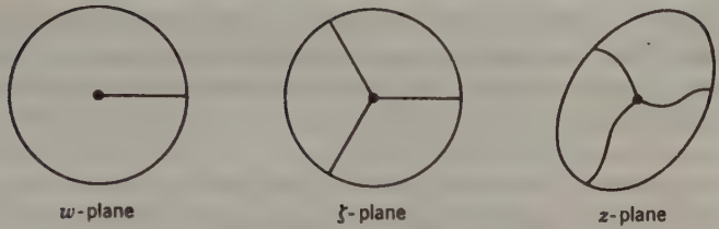
FIG. 4-8. Branch point: n = 3 .
