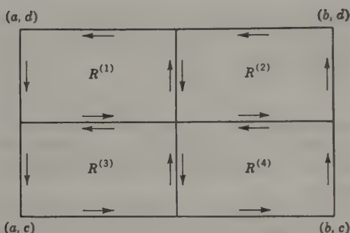
FIG. 4-2. Bisection of rectangle.
