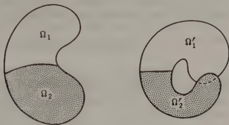
FIG. 3-1. Doubly covered region.
