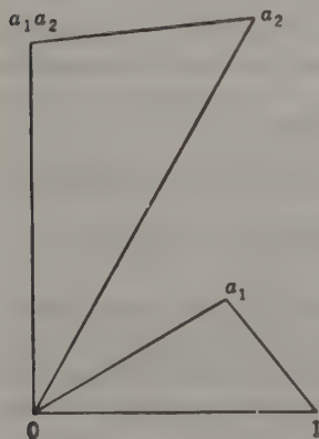
FIG. 1-2. Vector multiplication.
