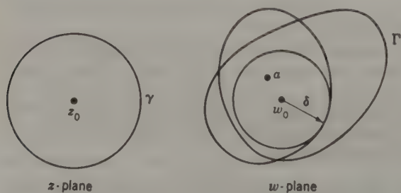
FIG. 4-7. Local correspondence.
