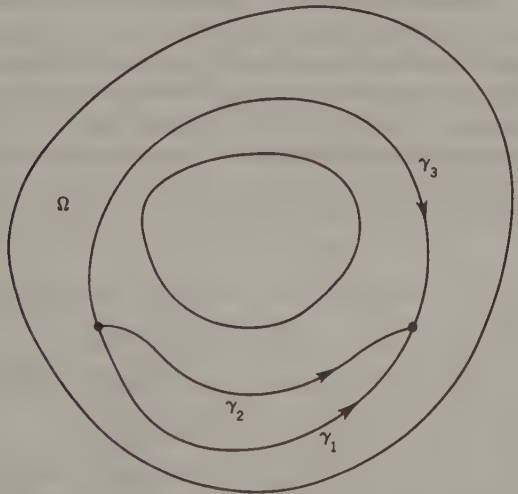
FIG. 8-1. Homotopic arcs.
