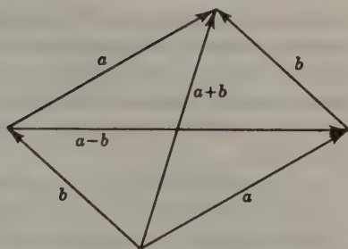
FIG. 1-1. Vector addition.
