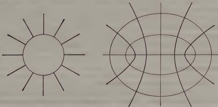
FIG. 3-9. Mapping by z = \frac{1}{2}(w + w^{-1}) .
