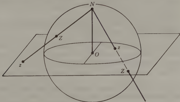
FIG. 1-3. Stereographic projection.
