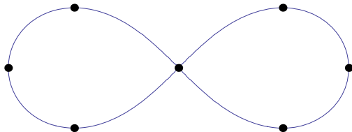
Figure 5.15. Lemniscate
