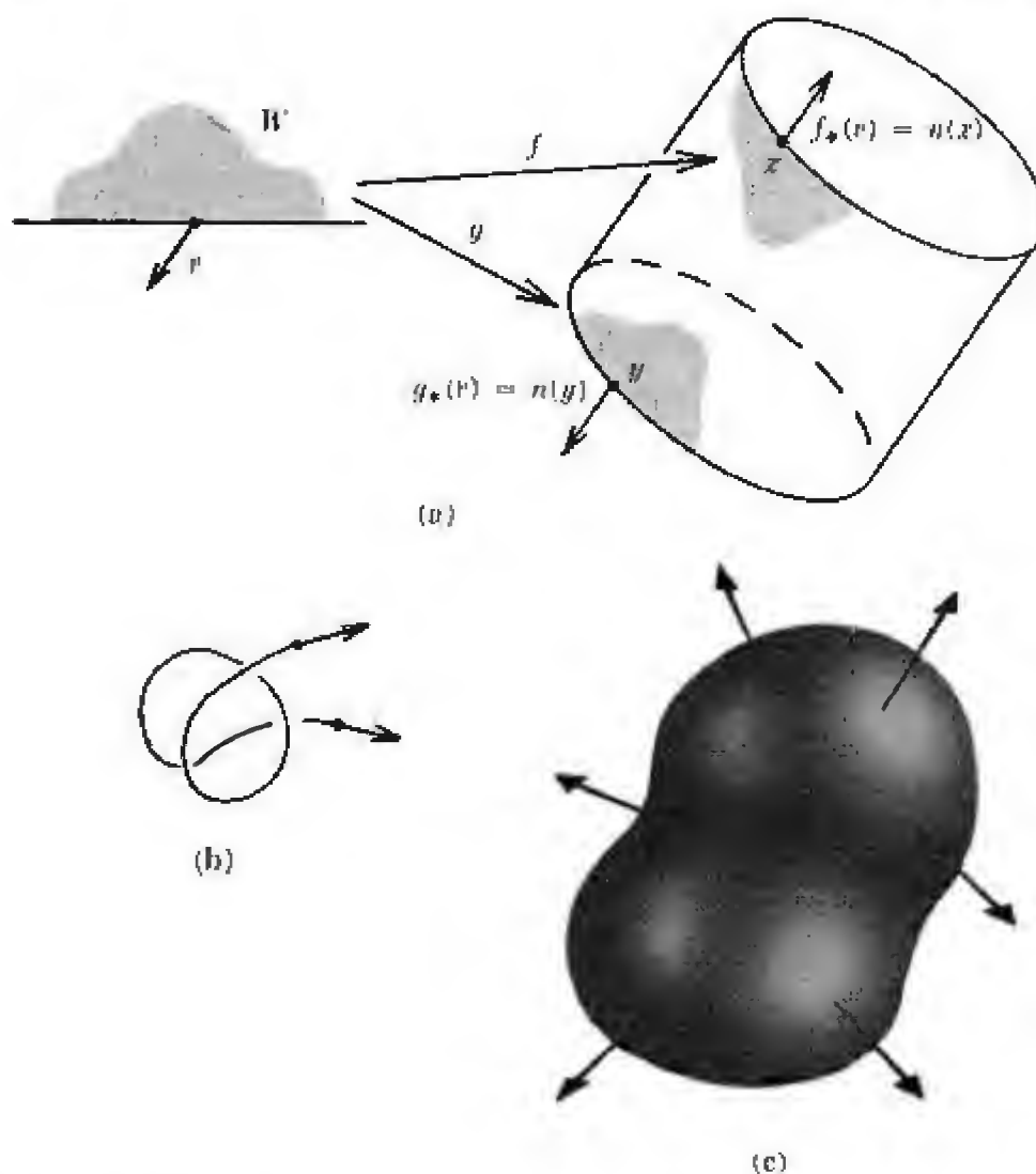
FIGURE 5-8. Some outward unit normal vectors of manifolds-with-boundary in \mathbf{R}^n .
