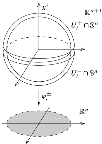
Fig. 1.3 Charts for \mathbb{S}^n
