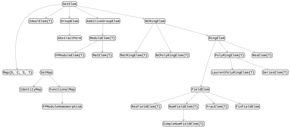
Figure 6.2: Diagram of element types
