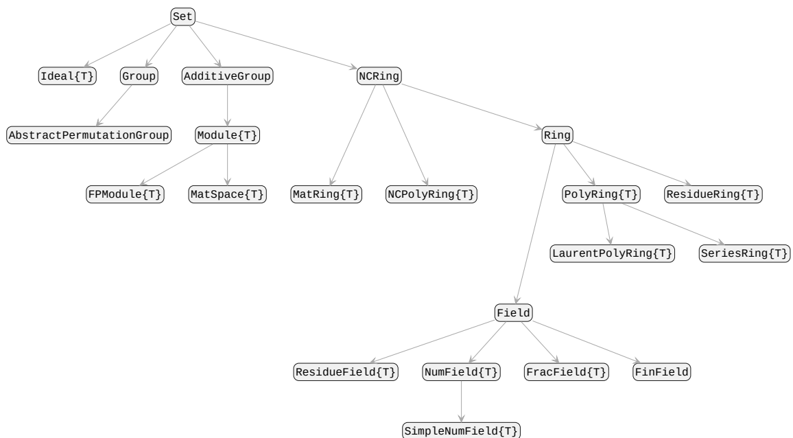
Figure 6.1: Diagram of parent types
