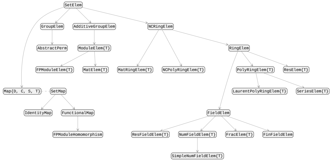
Figure 6.2: Diagram of element types
