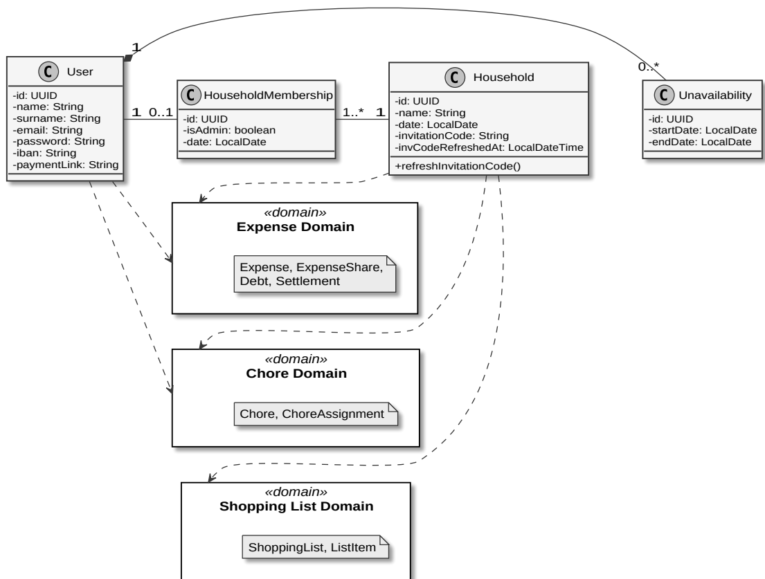
Figure 6.1: High-Level Backend Architecture Overview
