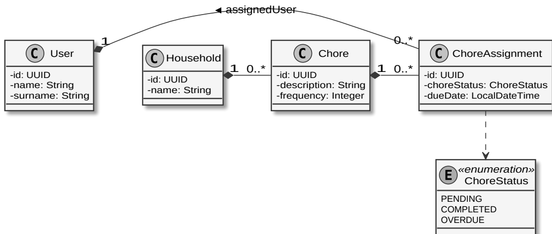
Figure 6.3: Chore Domain UML Class Diagram
