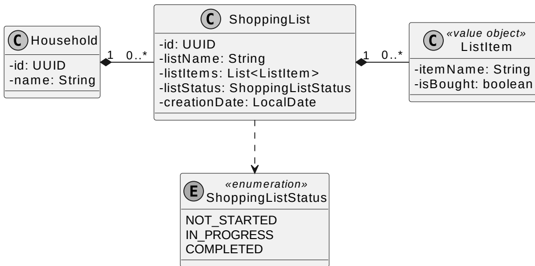
Figure 6.4: Shopping List Domain UML Class Diagram
