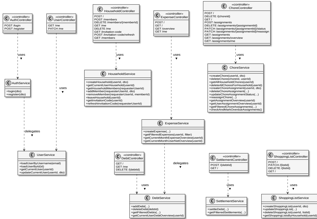
Figure 6.6: Controller and Service Layer UML Class Diagram
