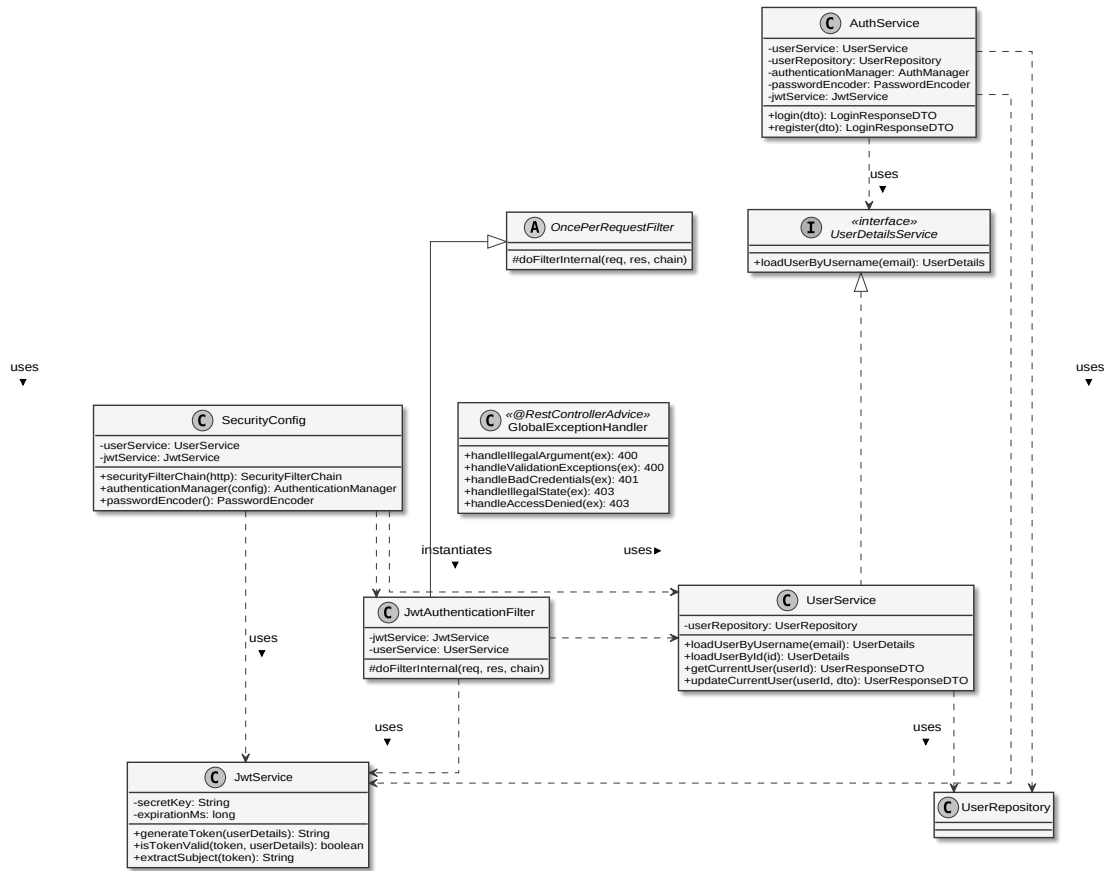
Figure 6.5: Authentication and Security UML Class Diagram
