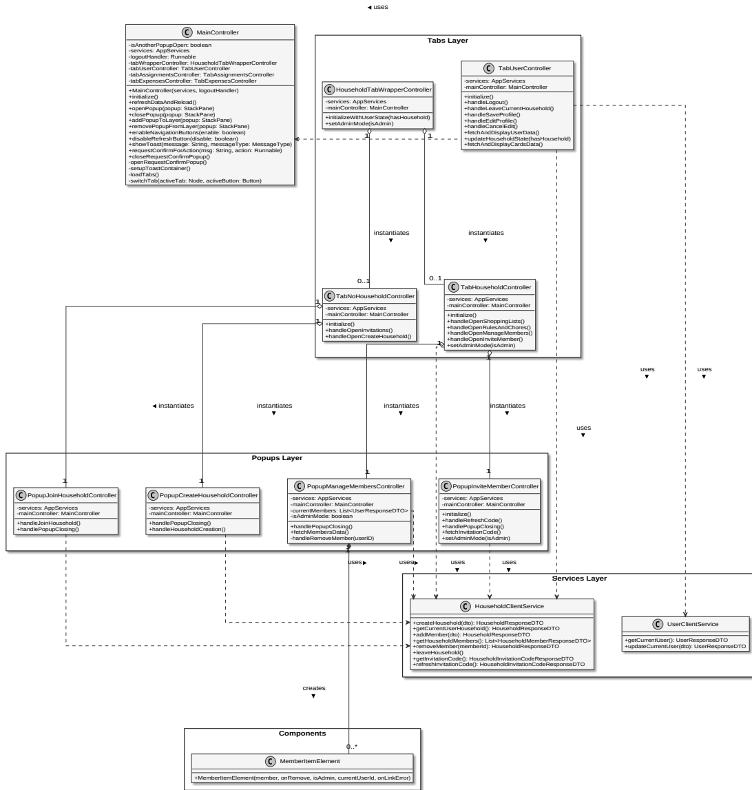
Figure 7.3: Client Module User-Household Domain UML Class Diagram
