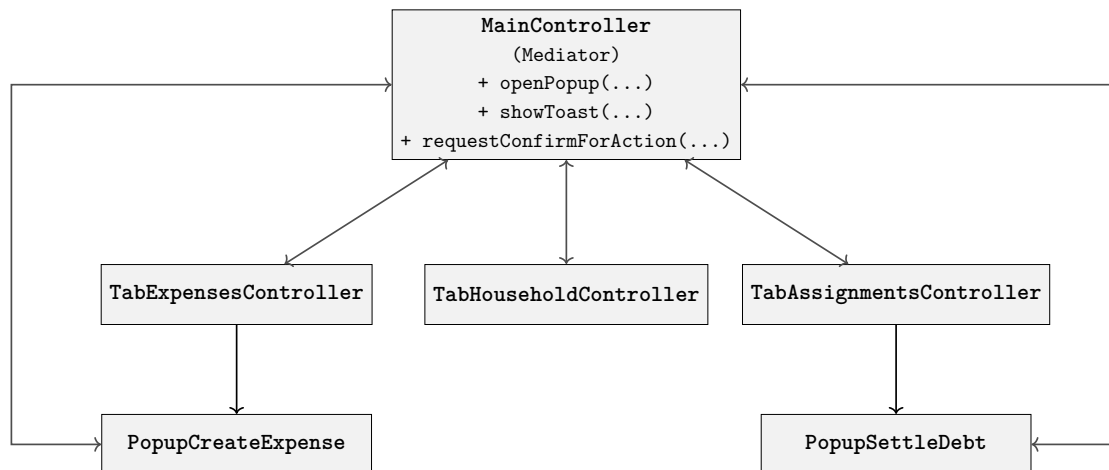
Figure 7.8: Mediator Pattern: Centralized UI Coordination
