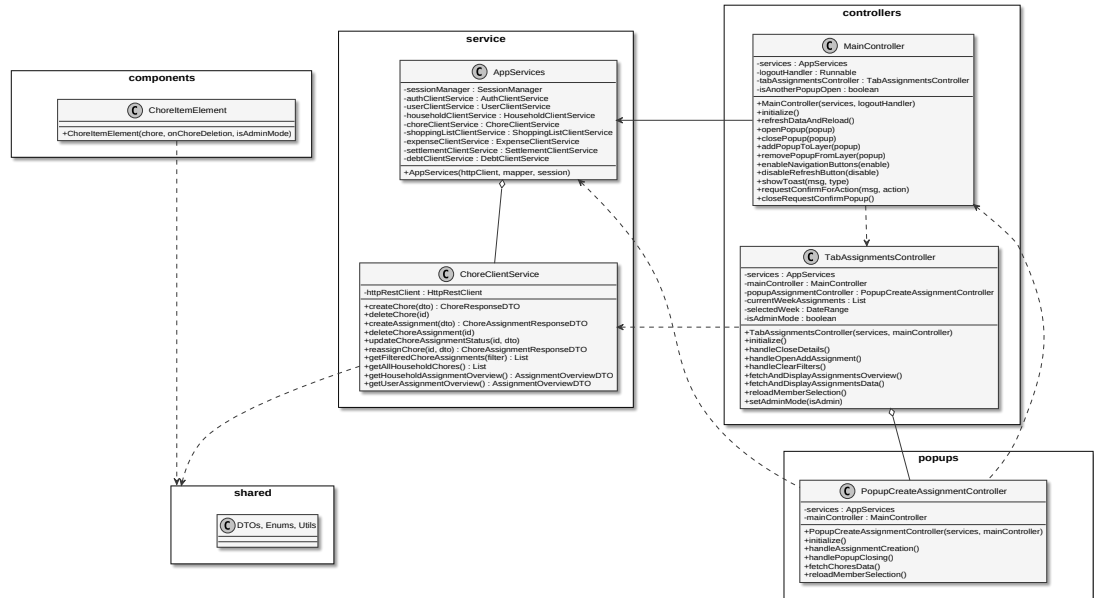
Figure 7.2: Client Module Chore Domain UML Class Diagram
