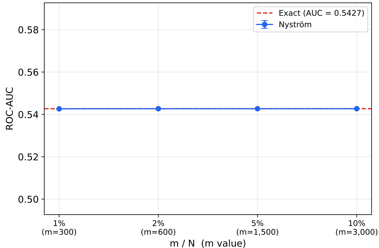
Downstream Task Performance (N = 30,000)
