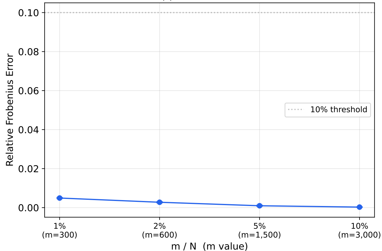
Kernel Approx. Error (N = 30,000)
