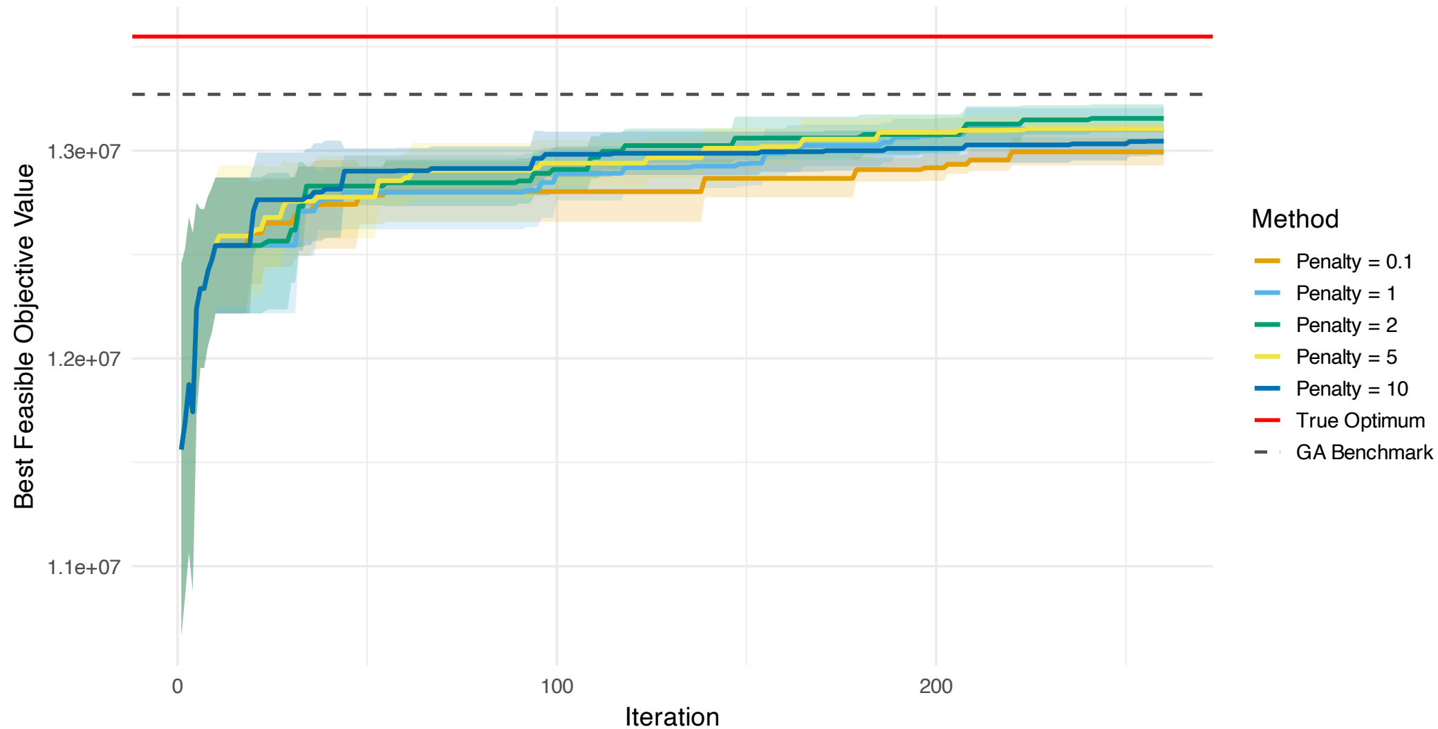
Optimisation Traces for BART-BO with different penalty weights
