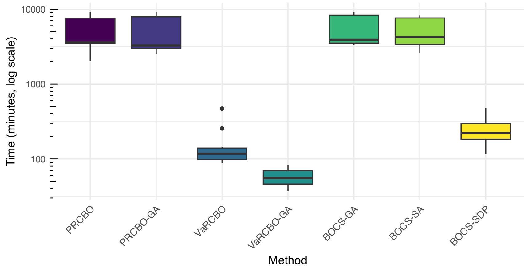
Execution Time Comparison (Log Scale)
