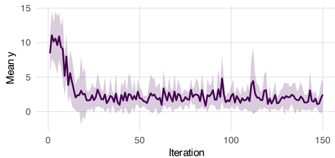
PRCBO-BFGS
