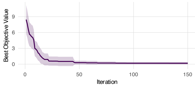
PRCBO-BFGS
