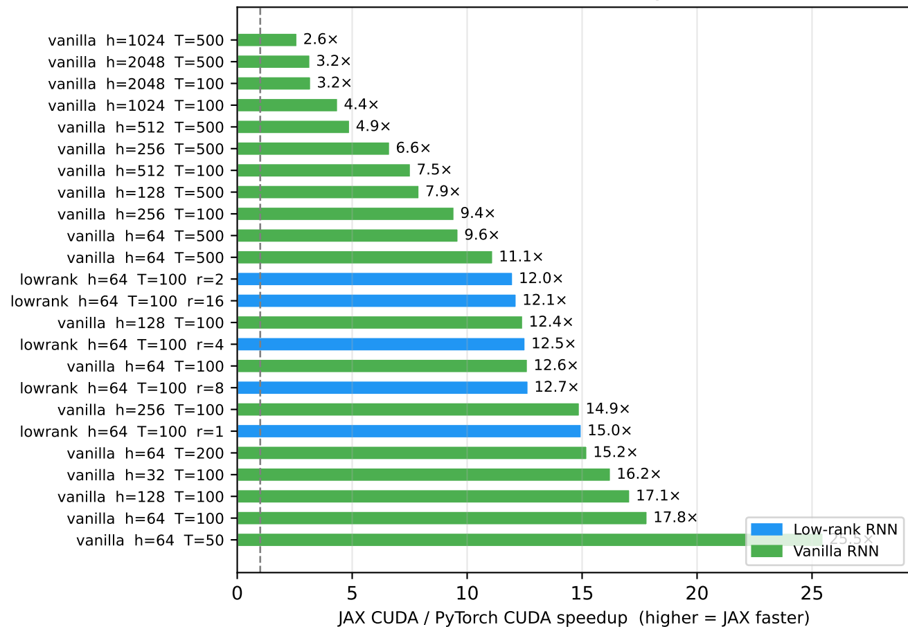
CUDA — JAX lax.scan vs PyTorch loop
