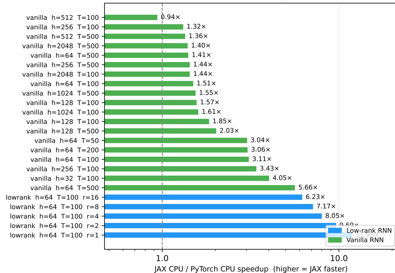
CPU — JAX lax.scan vs PyTorch loop
