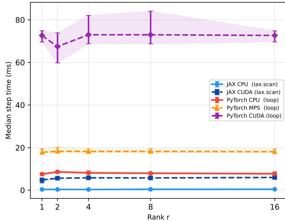
C Low-rank RNN — rank
