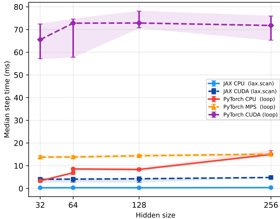
B Vanilla RNN — hidden size
