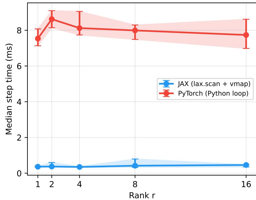
C Low-rank RNN — rank
