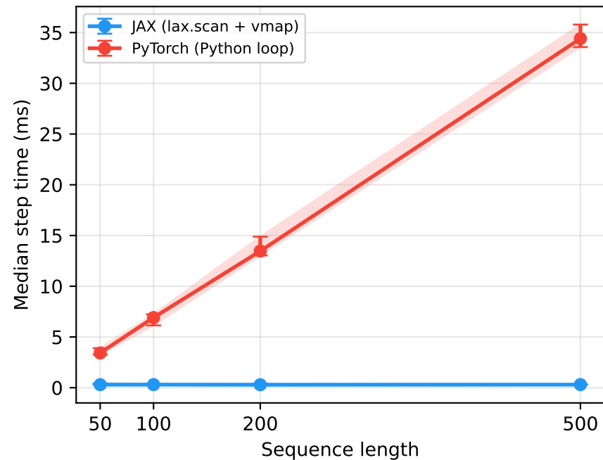
A Vanilla RNN — sequence length
