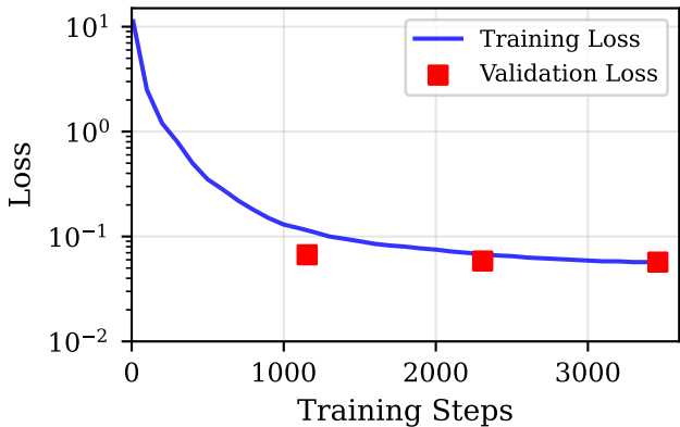
CodeT5 Training Convergence (Java→C#)
