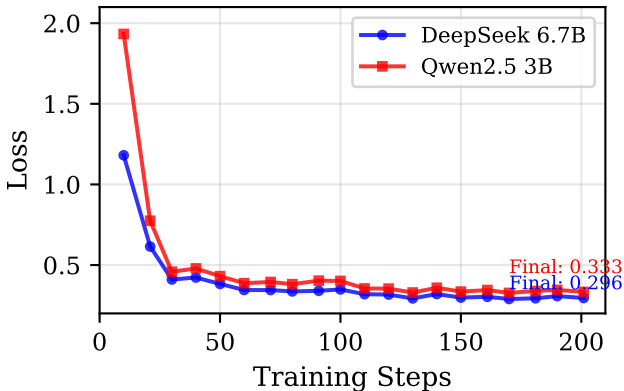
LoRA Fine-tuning Loss Curves
