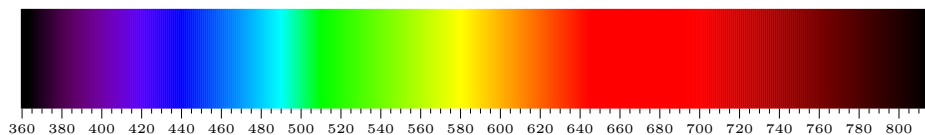
Figure 3.5: The visible light spectrum by wavelength, produced using xcolor , with units of nanometres.
