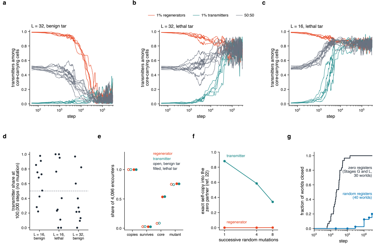
Extended Data Fig. 10 | The copy-offset switch and closure without supplied registers. a–c , A regenerator R and a transmitter T with the same core, XX\ 5e\ ed\ b0 , differing only in the offset byte and in what follows the core ( L = 32 : R = 04\ 5e\ ed\ b0 \times 8 , T = a0\ 5e\ ed\ b0 + 28 random bytes; L = 16 : R = 44\ 5e\ ed\ b0 \times 4 , T = b0\ 5e\ ed\ b0 + 12 random bytes, drawn for every cell), with the standard mutation: transmitters among the cells carrying the core against step, from 1% regenerators (vermillion), 1% transmitters (teal) or a 50:50 mixture (grey); one line per world (five, five and ten); samples with fewer than 1,000 core-carrying cells are omitted, and after step 5,000 each line is a running median of nine samples. At L = 32 every start converges to a low transmitter share with benign tar ( a ) and to a high one with lethal tar ( b ); at L = 16 with lethal tar ( c ) to a high one, although the core was later lost in 7 of 20 worlds (1 of 5 from 1% regenerators, 3 of 5 from 1% transmitters, 3 of 10 mixtures). At L = 16 with benign tar and mutation the core fell below 1,000 cells in all 20 worlds, and that condition is not shown. d , Without mutation the share drifts: transmitter share at 100,000 steps in each of ten 50:50 worlds per condition (dashed, the start). e , Encounter components of the pristine pair at L = 16 (4,096 encounters each; partners and executors drawn from the final soups of the mixed worlds of each tar, under benign tar soups in which the core had collapsed): exact copy into a partner (copies), exact survival as the partner of a soup executor (survives), core bytes 1–3 intact as a partner (core), and exact copying by a random single mutant (mutant); open, benign tar; filled, lethal tar. f , Post hoc, ref. 22's robustness criterion for the L = 32 pair (exact self-copy into the all-zero partner, 512 instructions, after k successive random mutations; 1,000 trials; median over 20 transmitter tails): the transmitter scores high because it keeps mutations, the regenerator near zero because it erases them. g , Closure at L = 16 with zero registers (black: fraction of the 30 worlds of Stages G and L whose first closed common tape has appeared) and with every register drawn at random before each encounter (blue: fraction of 40 worlds, seeds 8101–8120 and 8201–8220, in which most heritable cells among 64 random cells are confined, at the recorded snapshots); the two criteria differ, and the second is the stricter.
