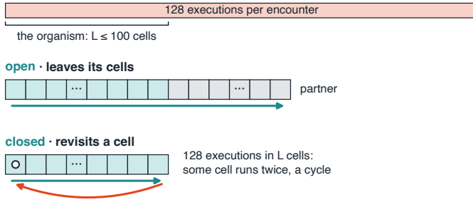
Fig. 6 | What is proved. a , Theorem 2 in the form that holds for the Z80 soups. An encounter executes 128 instructions, an organism has at most 100 cells, and no instruction stops execution inside it, so a program whose pointer never leaves its own cells (closed) must execute some cell twice, a cycle, whereas a program without one runs on into the partner (open). In BFF the same conclusion follows from the cost of a copy, at least 129 executions (Theorem 1). b , Proposition 3 with the count of Proposition 4. Of the 65,536 two-byte words, exactly five write themselves into an empty partner, all load–push pairs without a jump and therefore open, and no closed self-writer has period one or two; the smallest closer observed is the four-byte block copy 1e a4 ed b0 (LD E,n ; LDIR), whose LDIR repeats in place. Right, the chance that a given word is present among the 20,000 random tapes of length 16 at step 0: 0.99 for a two-byte word, 0.017 for a three-byte word and 6 \times 10^{-5} for a four-byte word. Proofs, the closure-window model and the lemma on information inflow are in the Supplementary Information.
