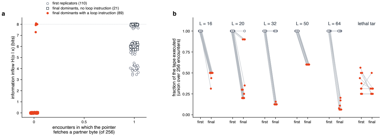
Extended Data Fig. 4 | Pointer confinement, information inflow and the executed part of the tape. Every first replicator and final dominant of Stages G, K and I (110 of each), run against 256 seeded random partners on a traced copy of the executor. a , Fraction of encounters in which the pointer fetches a partner byte against the information the offspring carry about the partner, H(o|x) (both jittered). The 100 first replicators born under benign tar enter the partner in every encounter and carry 3.4–8 bits; the ten born under lethal tar and all 89 loop-bearing final dominants never enter it, and 85 of the 89 carry no inflow, the other four keeping one to three partner bytes (7–8 bits); the 21 final dominants without a loop instruction are open pushers. b , Fraction of the tape fetched as instruction stream in any of the 256 encounters, first replicator against final dominant per world (grey lines join the same world; filled, loop instruction). The pusher executes its whole tape; the closers execute part of it and regenerate the rest.
