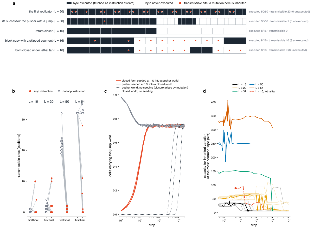
Fig. 4 | Closure wins the competition and inherits nothing. a , Where variation lives: for five genomes (the first replicator and the closed successor of one L = 50 world, the return design of L = 16, a block-copy tiling, and a lethal-tar final with a copied-but-unexecuted stretch), each byte is marked executed if the traced executor fetched it as instruction stream in any of 64 encounters, and transmissible if the mutational scan found at least half of its alternative values both heritable and transmitted; the pusher’s transmissible bytes are executed operands, the closers’ are bytes they copy but never run. b , Transmissible sites of the first replicator (first) against the final dominant (final) of every Stage G world, by tape length (grey lines join the same world; filled, loop instruction; open, none). c , The matched pair at L = 50: share of cells carrying the jump word 20 \pm 0 against step when the closed form is seeded at 1% into a world of its ancestor (five soups), when the ancestor is seeded into a world of the closed form (five) and in ancestor-only worlds with no seeding (three), in which the jump arises by mutation. d , Capacity for inherited variation of the most common tape against step ( \sum \log_2(1 + 255 f) over positions, bits), median over worlds: Stage G at L = 50 and 64, Stage K (L = 32), Stage I (L = 16, lethal tar) and the ten-million-step worlds of Stage L (L = 16 and 20), whose individual worlds are drawn as thin lines. Open marker, the first heritable dominant; filled marker, the first snapshot at which at least half of the dominants are pointer-closed. Capacity falls when closure arrives and stays low to ten million steps; at L = 20 the median alternates between open and closed worlds while closure spreads ( 10^5 – 10^6 steps). The thin peaks near 100 bits are the transient genomes of three worlds, block copiers whose transmissible sites are mostly never executed, each later displaced by a design with fewer sites or none.
