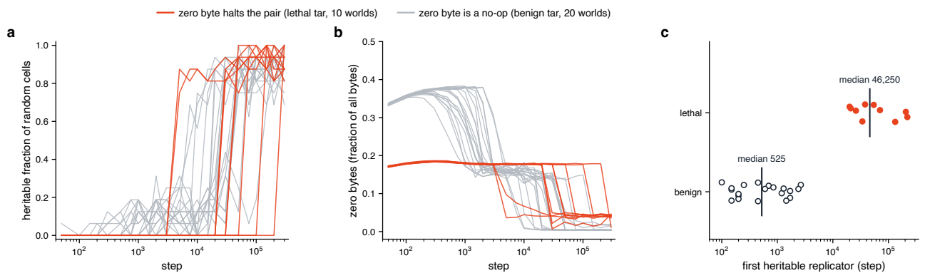
Extended Data Fig. 8 | Lethal tar in the first machine. Ten pre-registered worlds at L = 16 in which a zero byte fetched as an opcode halts the pair (Stage I, vermilion) against the twenty benign-tar worlds of Stage G at the same length (grey). a , Heritable fraction of 16 random cells against step. b , Zero-byte fraction against step. c , Step of the first heritable replicator in each world, with medians (46,250 against 525). Every lethal-tar first replicator is a block-copy replicator with a hardware loop, contains no zero byte, and copies 1.00 of partners with 0.00 self-damage from its first appearance.
