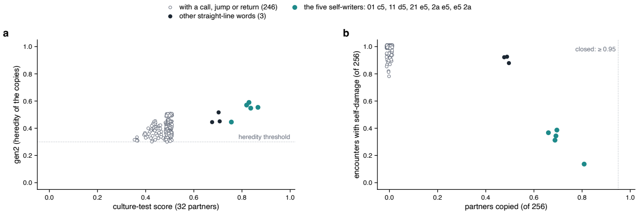
Extended Data Fig. 2 | Every two-byte word. All 65,536 two-byte words were tiled to 16 bytes and tested; shown are the 254 that pass the heredity threshold ( gen2 \geq 0.3 ). a , Culture-test score over 32 random partners against gen2 . The 246 words that contain a call, jump or return (open circles) pass by smearing return addresses into the partner; the five load-push words (teal) are exactly the words that write themselves into an all-zero partner (Proposition 3); the three other straight-line words (black) are their push-first rotations. b , The partner test over 256 random partners: fraction of partners that become \geq 75\% copy against the fraction of encounters in which the word loses a quarter or more of its own bytes. No word copies into 0.95 or more of partners, and none of the 246 produces a single 75% copy.
