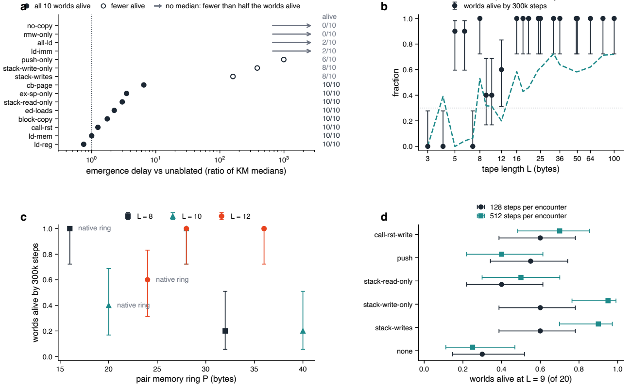
Extended Data Fig. 3 | What the instruction set must provide. a , Delay of emergence relative to the unablated soup (ratio of Kaplan–Meier medians, 128 steps, mutation 1/16, seeds 101–110) for each ablation; filled, all ten worlds alive; open, fewer; arrows, no ratio because fewer than half the worlds produced a replicator; right margin, worlds alive by 300,000 steps. b , Worlds alive by 300,000 steps against tape length (Wilson 95% intervals) and the first replicator's heritability in isolation (dashed; dotted line, the 0.3 threshold). c , Worlds alive against pair-memory ring length P at L = 8, 10, 12 (Stage F; the native ring is 2L): padding the ring without changing the organism removes the dead zone at L = 8–12. d , Worlds alive at L = 9 (of 20) by ablation at 128 and 512 steps per encounter (Stage D).
