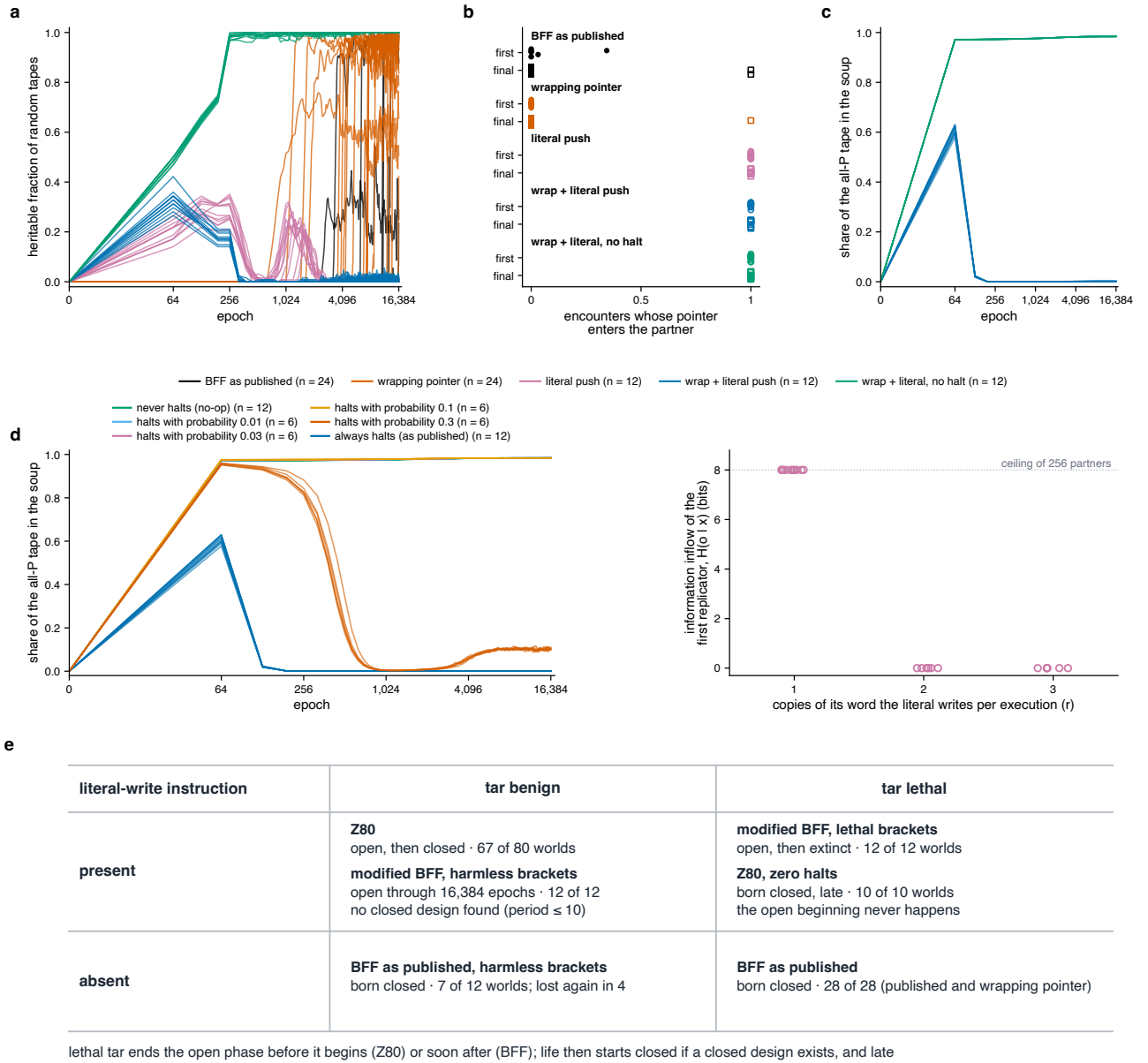
Fig. 5 | Two properties of the substrate decide the beginning. a , Heritable fraction of 32 random tapes against epoch for every BFF soup, by variant (as published, n = 24 ; wrapping pointer, n = 24 ; literal push, n = 12 ; wrap + literal push, n = 12 ; wrap + literal with unmatched brackets as no-ops, n = 12 ); the epoch axis is linear to 64 and logarithmic beyond, here and in c , d . b , Fraction of culture-test encounters in which the pointer enters the partner, for the first replicator (circles) and the final dominant (squares) of every life-producing soup, grouped by variant (open symbols, no loop instruction; filled, loop instruction). c , Share of the all-P class against epoch under wrap + literal (blue) and wrap + literal with no-op unmatched brackets (green), 12 worlds each (zero when the class is outside the ten largest): the same organism collapses when unmatched brackets halt the pointer and persists when they are no-ops. d , The two dials. Left, share of the all-P tape against epoch when an unmatched bracket halts the pointer with probability p = 0 (no-op, green), 0.01, 0.03, 0.1, 0.3 and 1 (as published, blue); 6 soups per intermediate p , 12 at the ends: the open replicator holds the soup at p \leq 0.1 , collapses to a tenth of it at p = 0.3 and to a 0.2% minority at p = 1 . Right, information inflow of the first replicator, H(o|x) (bits) over 256 random partners, when the literal writes r = 1, 2 or 3 copies of its word per execution (one point per soup; open symbols, no loop): at r \geq 2 a copy completes within one pass and the offspring carry nothing of the partner although the pointer still enters it. e , Map of the substrates by two properties, a literal-write instruction (present or absent) and the lethality of the tar to an open replicator, with the observed order of events and world counts in each cell: with a literal channel and benign tar, life begins open and closes (the Z80, its 8080 subset at L = 16 , and BFF with no-op brackets, which stays open); with a literal channel and lethal tar, the Z80 skips the open beginning and starts closed and late, and BFF's brief open beginning ends in extinction; without a literal channel BFF is born closed, and with harmless brackets loses the replicator again in 4 of 7 soups.
