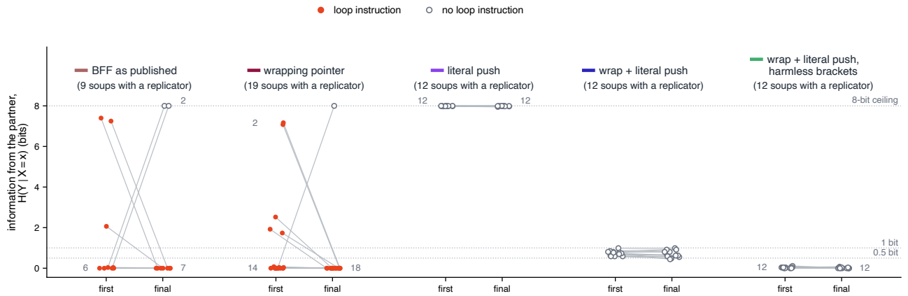
Supplementary Fig. 2 | Information inflow in the second machine. H(Y|X=x) over 256 random partners for the first replicator and the final dominant of every BFF soup with a replicator, by variant (grey lines join the same soup; filled, both brackets present, a loop; numbers, coincident points; the bar before each name, the variant's colour in Fig. 5), with the 8-bit ceiling of 256 partners and the 1-bit and 0.5-bit thresholds registered for the inflow analysis (Supplementary Methods, Pre-registration and stages). Without a literal channel (as published, and with a wrapping pointer) every first replicator carries a loop and most carry no inflow; the literal push without a wrapping pointer sits at the ceiling; under a wrapping pointer the literal tiling floods the ring and carries less than 1 bit, with harmless brackets at most 0.11, although its pointer enters the partner in every encounter. The loop-free finals at the 8-bit ceiling are the literal pushers without a wrapping pointer, open copiers (11 of 12 copy 89–94% of partners, the twelfth none) that lie outside Theorem 1, which concerns published BFF programs whose pointer stays in their own cells, and three one-symbol fills (two as published, one with a wrapping pointer) that had displaced the replicator and copy 0.00–0.02 of partners.
