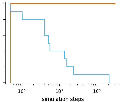
Time to first replicator, L = 100 bytes (Kaplan-Meier; ticks = censored at the run's last step) 128 steps · mutation 1/2^4
