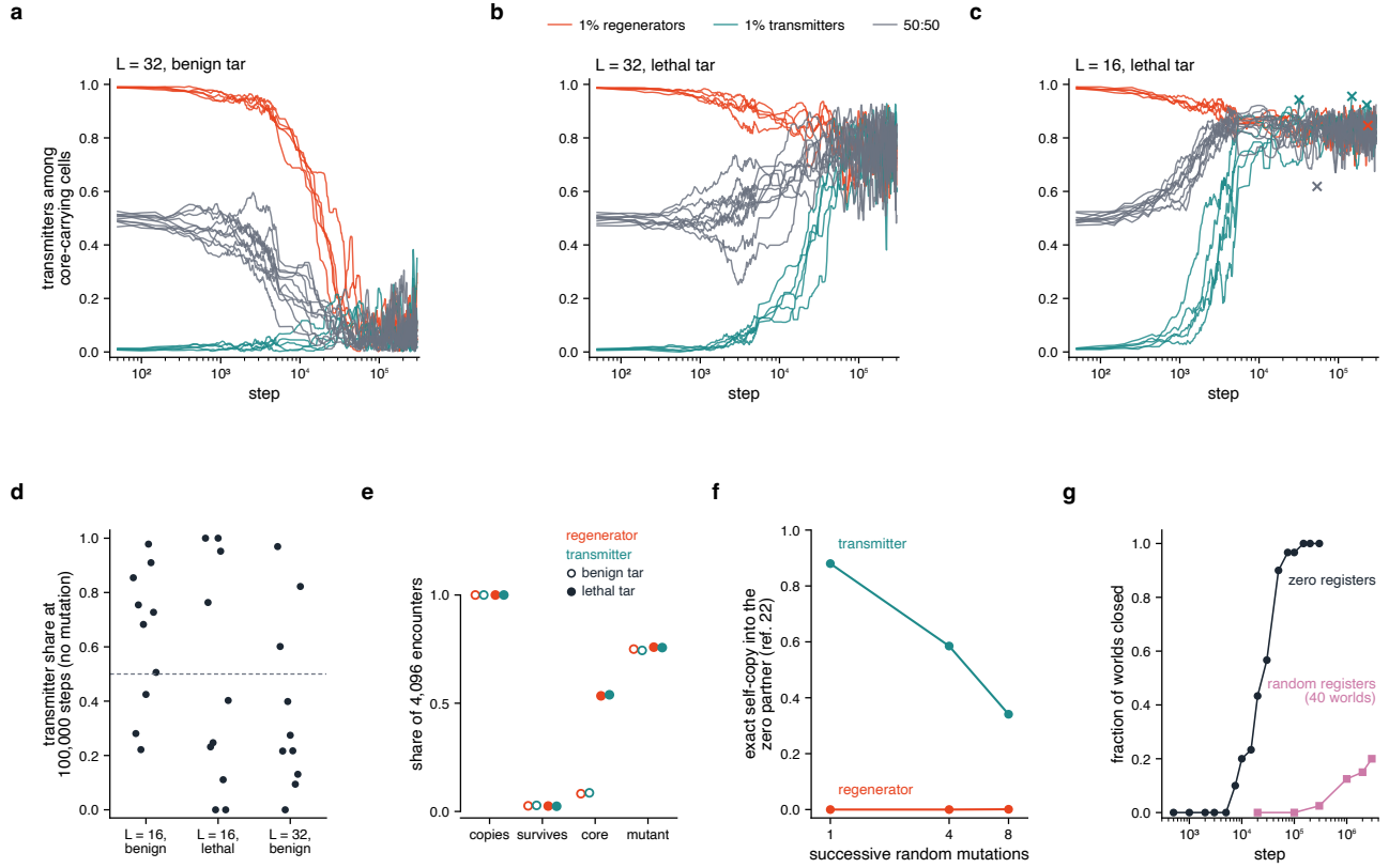
Extended Data Fig. 10 | The copy-offset switch and closure without supplied registers. a–c, A regenerator R and a transmitter T with the same core, XX\ 5e\ ed\ b0 , differing only in the offset byte and in what follows the core (L = 32: R = 04\ 5e\ ed\ b0 \times 8 , T = a0\ 5e\ ed\ b0 + 28 random bytes; L = 16: R = 44\ 5e\ ed\ b0 \times 4 , T = b0\ 5e\ ed\ b0 + 12 random bytes, drawn for every cell), with the standard mutation: transmitters among the cells carrying the core against step, from 1% regenerators (vermillion), 1% transmitters (teal) or a 50:50 mixture (grey); one line per world (five, five and ten); after step 5,000 each line is a running median of nine samples, and samples with fewer than 1,000 core-carrying cells are then omitted; x, the last sample before a world lost the core. At L = 32 every start converges to a low transmitter share with benign tar (a) and to a high one with lethal tar (b); at L = 16 with lethal tar (c) to a high one, although the core was later lost in 7 of 20 worlds (1 of 5 from 1% regenerators, 3 of 5 from 1% transmitters, 3 of 10 mixtures). At L = 16 with benign tar and mutation the core fell below 1,000 cells in all 20 worlds, and that condition is not shown; 7 of the 20 were above 1,000 again at 300,000 steps, with transmitter shares of 0.14–0.63. d, Without mutation the share drifts: transmitter share at 100,000 steps in each of ten 50:50 worlds per condition (dashed, the start). e, Encounter components of the pristine pair at L = 16 (4,096 encounters each; partners and executors drawn from the final soups of the mixed worlds of each tar, under benign tar soups in which the core had collapsed): exact copy into a partner (copies), exact survival as the partner of a soup executor (survives), core bytes 1–3 intact as a partner (core), and exact copying by a random single mutant (mutant); hollow markers, benign tar; filled, lethal tar. f, Post hoc, ref. 22's robustness criterion for the L = 32 pair (exact self-copy into the all-zero partner, 512 instructions, after k successive random mutations; 1,000 trials; median over 20 transmitter tails): the transmitter scores high because it keeps mutations, the regenerator near zero because it erases them. g, Fraction of worlds at L = 16 in which most heritable cells among 64 random cells are confined, at the recorded snapshots, with zero registers (black: Stages G and L, 30 worlds; 20 at 7,500 steps) and with every register drawn at random before each encounter (pink: 40 worlds, seeds 8101–8120 and 8201–8220).
