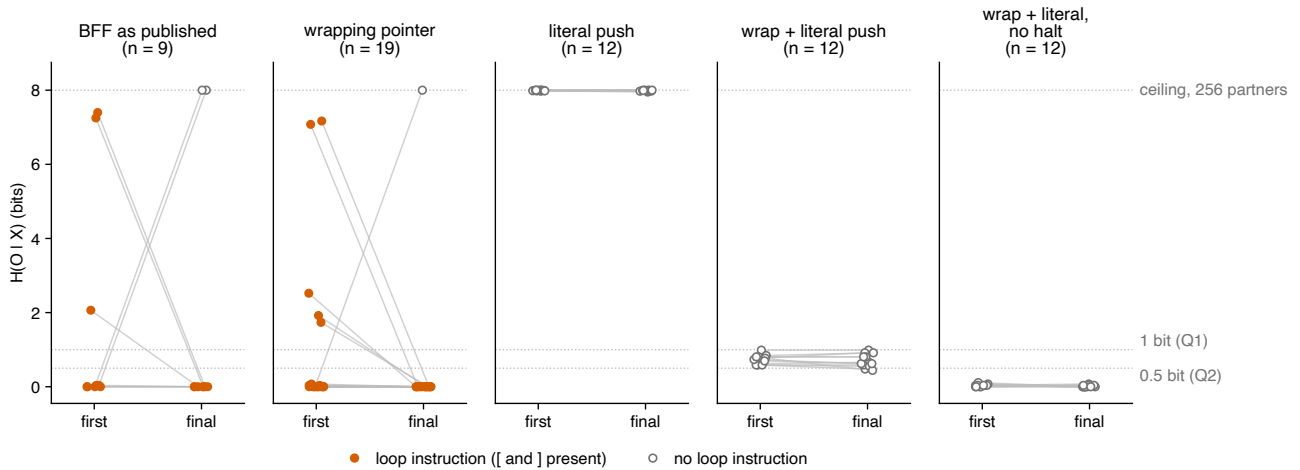
Extended Data Fig. 8 | Searches and information inflow in BFF. The 16.4-million-program straight-line search under a wrapping pointer (copy fraction and offspring byte diversity of the 130 programs passing the byte-match criterion) and the 1.3-million-tiling closed-replicator search under the benign-tar rule (open replicators by period; no closed heritable tiling). H(o | x) over 256 random partners for the first replicator and the final dominant of every life-producing BFF soup, by variant (lines join the same soup; filled, both brackets present), with the 8-bit ceiling of 256 partners and the pre-registered 1-bit and 0.5-bit thresholds. The published variant is born with near-zero inflow; the literal-push variant without a wrapping pointer sits at the ceiling; the two wrapping literal variants flood the ring and have near-zero inflow although their pointer enters the partner in every encounter.
