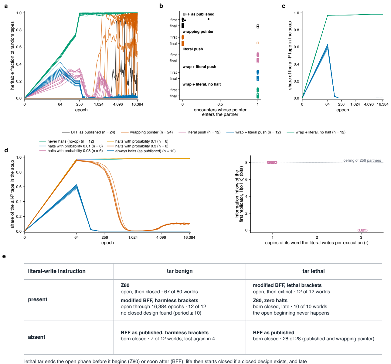
Fig. 5 | Two properties of the substrate decide the beginning. a , Heritable fraction of 32 random tapes against epoch for every BFF soup, by variant (as published, n = 24 ; wrapping pointer, n = 24 ; literal push, n = 12 ; wrap + literal push, n = 12 ; wrap + literal with unmatched brackets as no-ops, n = 12 ); the epoch axis is linear to 64 and logarithmic beyond, here and in c , d . b , Fraction of culture-test encounters in which the pointer enters the partner, for the first replicator (circles) and the final dominant (squares) of every life-producing soup, grouped by variant (open symbols, no loop instruction; filled, loop instruction). c , Share of the all-P class against epoch under wrap + literal (blue) and wrap + literal with no-op unmatched brackets (green), 12 worlds each (zero when the class is outside the ten largest): the same organism collapses when unmatched brackets halt the pointer and persists when they are no-ops. d , The two dials. Left, share of the all-P tape against epoch when an unmatched bracket halts the pointer with probability p = 0 (no-op, green), 0.01, 0.03, 0.1, 0.3 and 1 (as published, blue); 6 soups per intermediate p , 12 at the ends: the open replicator holds the soup at p \leq 0.1 , collapses to a tenth of it at p = 0.3 and to a 0.2% minority at p = 1 . Right, information inflow of the first replicator, H(o|x) (bits) over 256 random partners, when the literal writes r = 1, 2 or 3 copies of its word per execution (one point per soup; open symbols, no loop): at r \geq 2 a copy completes within one pass and the offspring carry nothing of the partner although the pointer still enters it. e , Map of the substrates by two properties, a literal-write instruction (present or absent) and the lethality of the tar to an open replicator, with the observed order of events and world counts in each cell: with a literal channel and benign tar, life begins open and closes (the Z80, its 8080 subset at L = 16 , and BFF with no-op brackets, which stays open); with a literal channel and lethal tar, the Z80 skips the open beginning and starts closed and late, and BFF's brief open beginning ends in extinction; without a literal channel BFF is born closed, and with harmless brackets loses the replicator again in 4 of 7 soups.
