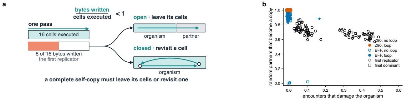
Fig. 5 | Closure as a cycle. a , Theorem 2 as a diagram. A program that writes fewer bytes than the cells it executes cannot copy itself in one pass: the first replicator ( L = 16 ) executes its 16 cells and has written 8 of the 16 bytes a copy needs (executor trace), so copying requires more execution, which can only continue outside its cells (open) or revisit one of them (closed, a cycle). b , Copy success against self-damage for every measured first (circles) and final (squares) replicator: Z80 (black/vermilion) and BFF (blue); filled, loop-bearing. The closure-window model ( q \int n \, dt ) is in Extended Data.
