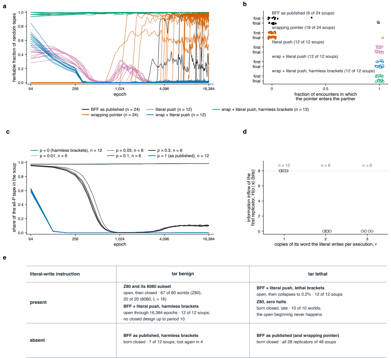
Fig. 5 | Two properties of the substrate decide the beginning. a , Heritable fraction of 32 random tapes against epoch for every BFF soup, by variant: as published (n = 24), with a wrapping pointer (24), with the literal push (12), with both (12), and with both and harmless brackets, which are no-ops instead of halting the pointer (12); samples every 64 epochs from epoch 64. b , Fraction of culture-test encounters in which the pointer enters the partner, for the first replicator (circles) and the final dominant (squares) of every soup with life, by variant (open symbols, no loop instruction; filled, loop instruction; jittered). c , Lethality as a dial: share of the all-P tape, the literal instruction tiled, against epoch under wrap + literal push when an unmatched bracket halts the pointer with probability p (p = 0, 12 soups; 0.01, 0.03, 0.1 and 0.3, six each; 1, as published, 12); the curves for p \leq 0.1 lie on top of one another near 1. d , The write ratio: information inflow of the first replicator, H(o | x) over 256 random partners (dotted line, the 8-bit ceiling), when the literal push without a wrapping pointer writes r = 1, 2 or 3 copies of its word per execution; one point per soup, every first replicator loop-free. e , The map: the observed order of events in each cell defined by a literal-write instruction (present or absent) and by the lethality of the tar to an open replicator, with world counts.
