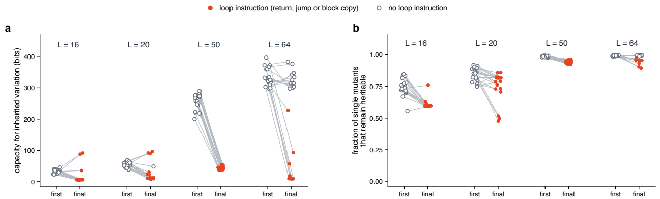
Supplementary Fig. 2 | Single-mutant scan of first and final dominants. Single-byte mutational scan of the first heritable replicator (first) and the final dominant (final) of every Stage G world, grouped by tape length (grey lines join the same world; filled, loop instruction; open, none); transmission is scored in first-generation copies; serial transfers are in Fig. 4a–c. a , Single-mutant variation score, \sum \log_2(1 + 255 \times \text{fraction of transmissible values}) over positions, in bits. b , Robustness: fraction of single mutants that remain heritable ( \text{gen2} \geq 0.3 ). All 255 alternative bytes per position at L = 16 and 20, 32 seeded values at L = 50 and 64; 32 partners per generation.
