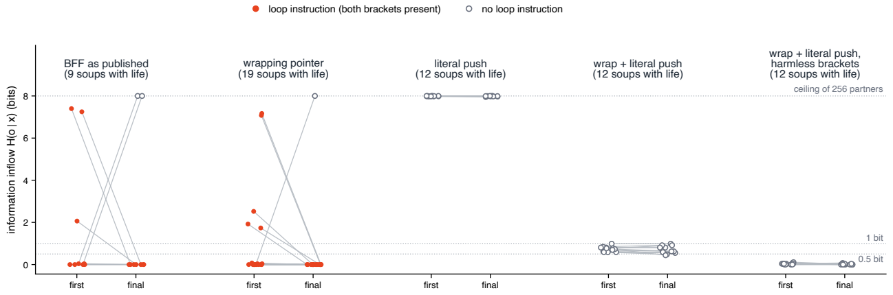
Supplementary Fig. 3 | Information inflow in the second machine. H(Y | X = x) over 256 random partners for the first replicator and the final dominant of every life-producing BFF soup, by variant (grey lines join the same soup; filled, both brackets present, a loop), with the 8-bit ceiling of 256 partners and the pre-registered 1-bit and 0.5-bit thresholds. Without a literal channel (as published, and with a wrapping pointer) every first replicator carries a loop and most carry no inflow; the literal push without a wrapping pointer sits at the ceiling; under a wrapping pointer the literal tiling floods the ring and carries less than 1 bit, with no-op brackets at most 0.11, although its pointer enters the partner in every encounter. The loop-free finals at the 8-bit ceiling are the literal pushers without a wrapping pointer, open copiers (11 of 12 copy 89–94% of partners, the twelfth none) that lie outside Theorem 1, which concerns published BFF programs whose pointer stays in their own cells, and three one-symbol fills (two as published, one with a wrapping pointer) that had displaced the replicator and copy 0.00–0.02 of partners.
