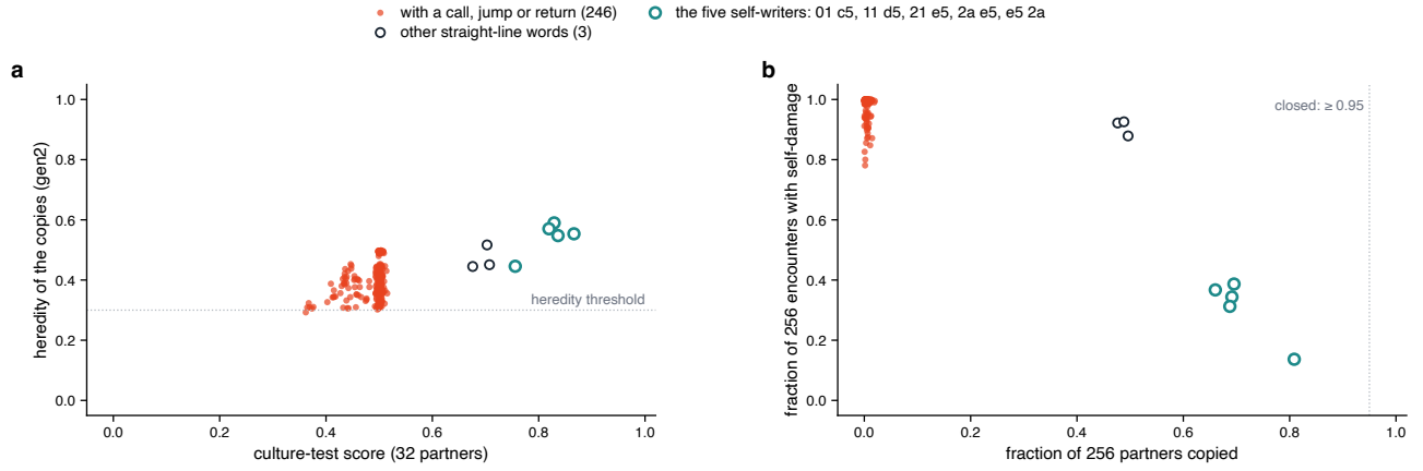
Supplementary Fig. 1 | Every two-byte word. All 65,536 two-byte words were tiled to 16 bytes and tested; shown are the 254 that pass the hereditary threshold ( \text{gen2} \geq 0.3 ). a , The hereditary of the copies ( \text{gen2} ) against the culture-test score over 32 random partners. The 246 words that contain a call, jump or return (vermillion) pass by smearing return addresses into the partner: \text{gen2} is a normalised gain in best-shift similarity to the original tape, so smeared return addresses raise the partners' similarity to the word without making copies, and hereditary is read together with the copies of the partner test (b). The five load-push words (teal) are exactly the words, besides the trivial 00 00, that write themselves into an all-zero partner (Proposition 3); the three other straight-line words (black) are their push-first rotations. b , The partner test over 256 random partners: the fraction of encounters in which the word loses a quarter or more of its own bytes against the fraction of partners that become a \geq 75\% copy; dotted line, the 0.95 that defines a closed copier. No word reaches it, and none of the 246 produces a single 75% copy. Coincident points are spread by a small one-sided jitter.
