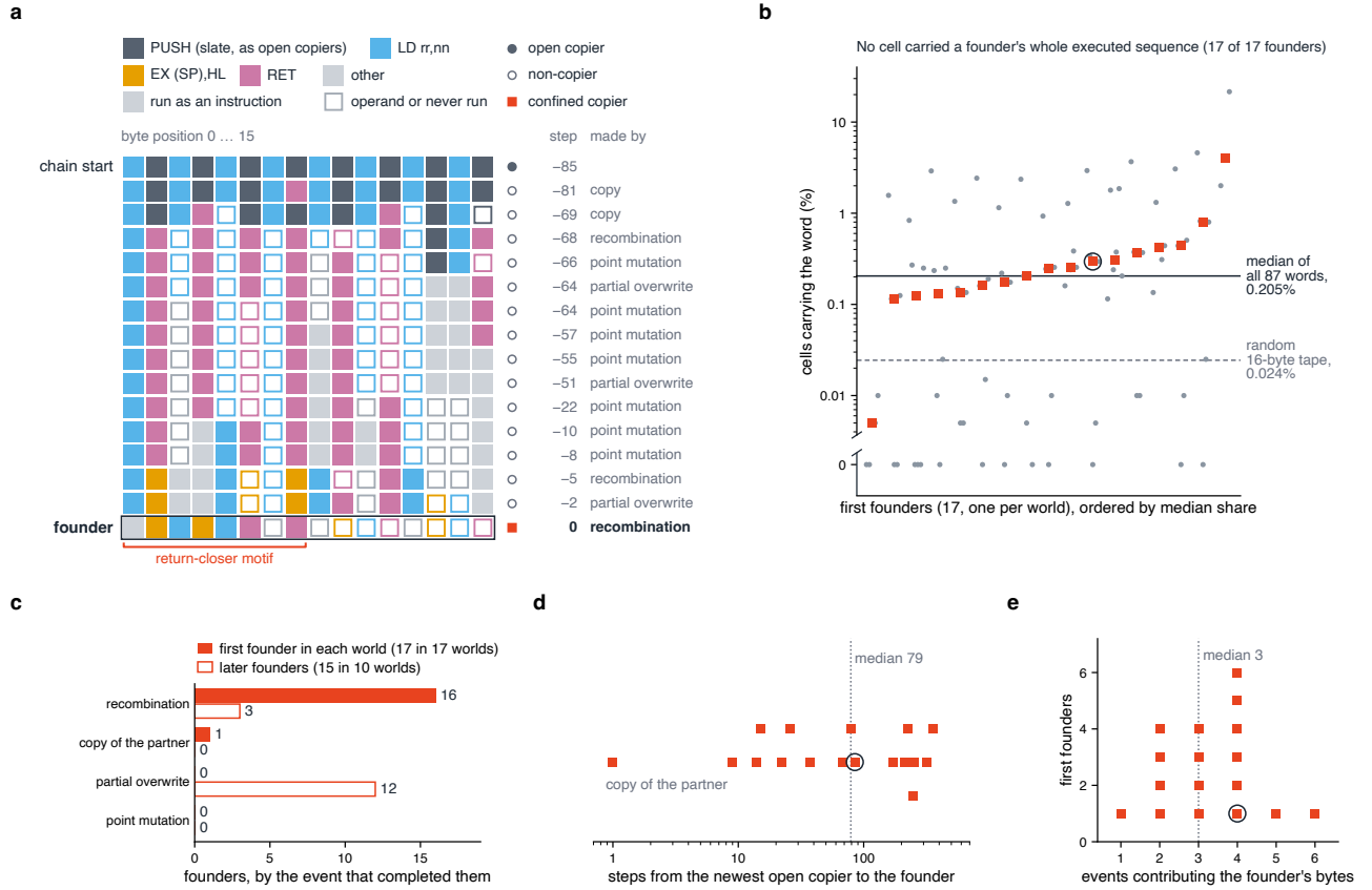
Extended Data Fig. 7 | The first self-confined copier of each world was completed by recombination, from parts circulating in non-copiers. a , The line of descent in world 31010 (the chain closest to the median, 14 records over 79 steps), from the newest open copier older than the founder (chain start) to the founder (boxed); each row is a record, with its step relative to the founder and the event that made it. Bytes are coloured by value (PUSH slate, the open-copier colour); a filled byte is an instruction start in at least half of 64 encounters with random partners, an outlined byte only an operand or never run; markers give each tape's class against the same partners. The half of the founder that runs is the return-closer motif. b , For each of the 17 first founders, the share of the 20,000 cells carrying each two-byte word that begins at one of its instruction starts (grey; 87 words) in the last soup snapshot before the founder; squares, each founder's median; ring, the world in a ; solid line, the median of all words; dashed, the expectation for a random 16-byte tape. Words carried by no cell (15 of 87) are drawn below the break; no cell carried any founder's whole executed sequence. c , The event that completed each founder: first founders (filled; one in each of 17 worlds) and later founders in the same worlds (open; 15 in 10 worlds). d , Steps from the newest open copier to each first founder. e , Distinct events that set the founder's bytes. Recombination: the new tape keeps less than 75% of its own bytes and is not a \geq 75\% copy of its partner; partial overwrite: it keeps at least 75%; copy of the partner: it becomes a \geq 75\% copy of its partner; point mutation: the simulator's mutation operator. Exploratory: the chain start, the separation of first from later founders and the word measure were defined after the recorded lines were inspected (Methods).
