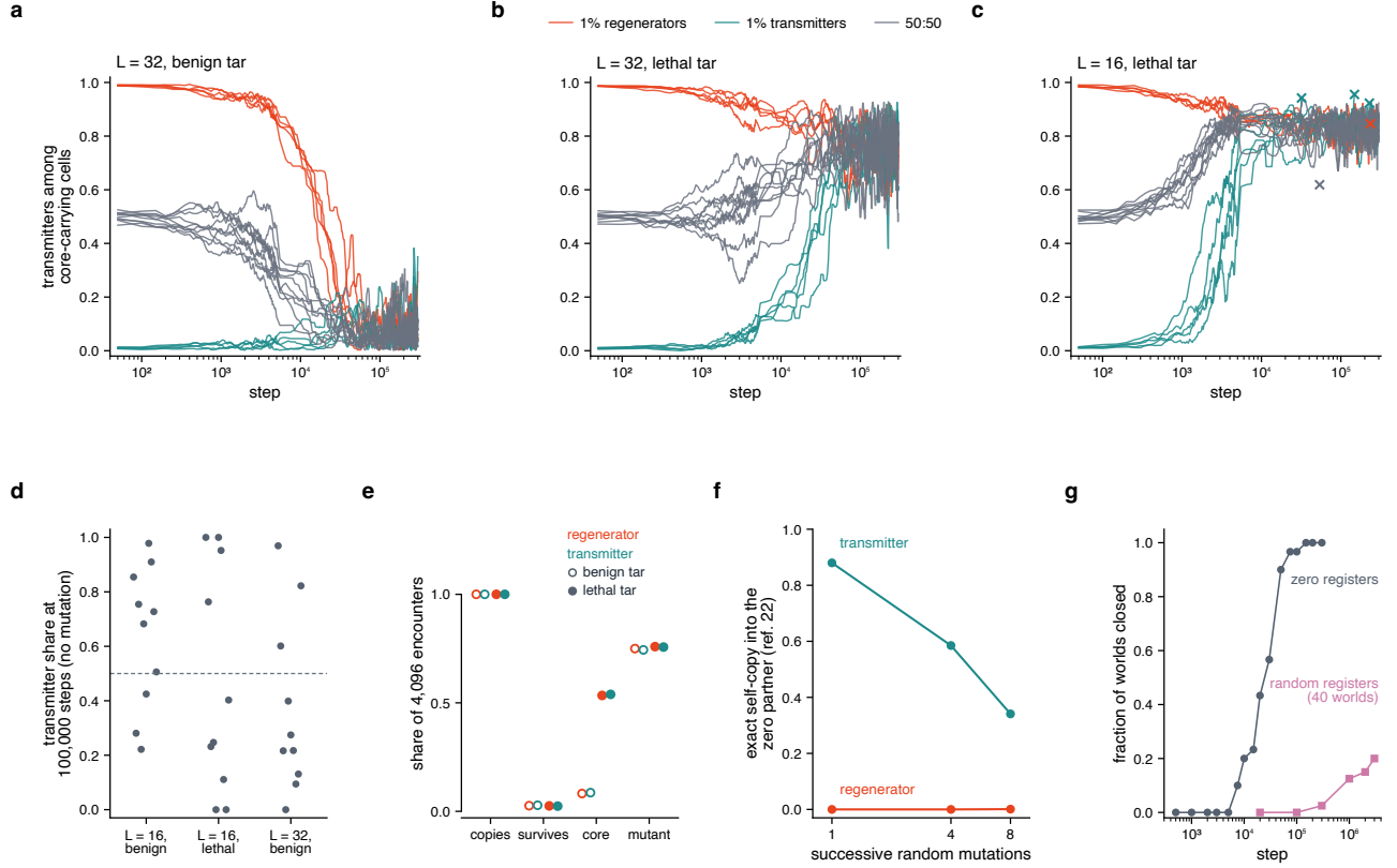
Extended Data Fig. 6 | The copy-offset switch and closure without supplied registers. a–c , A regenerator R and a transmitter T with the same core, XX\ 5e\ ed\ b0 , differing only in the offset byte and in what follows the core ( L = 32 : R = 04\ 5e\ ed\ b0 \times 8 , T = a0\ 5e\ ed\ b0 + 28 random bytes; L = 16 : R = 44\ 5e\ ed\ b0 \times 4 , T = b0\ 5e\ ed\ b0 + 12 random bytes, drawn for every cell), with the standard mutation: transmitters among the cells carrying the core against step, from 1% regenerators (vermillion), 1% transmitters (teal) or a 50:50 mixture (grey); one line per world (five, five and ten); after step 5,000 each line is a running median of nine samples, and samples with fewer than 1,000 core-carrying cells are then omitted; \times , the last sample before a world lost the core. At L = 32 every start converges to a low transmitter share with benign tar (a) and to a high one with lethal tar (b); at L = 16 with lethal tar (c) to a high one, although the core was later lost in 7 of 20 worlds (1 of 5 from 1% regenerators, 3 of 5 from 1% transmitters, 3 of 10 mixtures). At L = 16 with benign tar and mutation the core fell below 1,000 cells in all 20 worlds, and that condition is not shown; 7 of the 20 were above 1,000 again at 300,000 steps, with transmitter shares of 0.14–0.63. d , Without mutation the share drifts: transmitter share at 100,000 steps in each of ten 50:50 worlds per condition (dashed, the start). e , Encounter components of the pristine pair at L = 16 (4,096 encounters each; partners and executors drawn from the final soups of the mixed worlds of each tar, under benign tar soups in which the core had collapsed): exact copy into a partner (copies), exact survival as the partner of a soup executor (survives), core bytes 1–3 intact as a partner (core), and exact copying by a random single mutant (mutant); hollow markers, benign tar; filled, lethal tar. f , Post hoc, ref. 22's robustness criterion for the L = 32 pair (exact self-copy into the all-zero partner, 512 instructions, after k successive random mutations; 1,000 trials; median over 20 transmitter tails): the transmitter scores high because it keeps mutations, the regenerator near zero because it erases them. g , Fraction of worlds at L = 16 in which most heritable cells among 64 random cells are confined, at the recorded snapshots, with zero registers (slate: Stages G and L, 30 worlds; 20 at 7,500 steps) and with every register drawn at random before each encounter (pink: 40 worlds, seeds 8101–8120 and 8201–8220).
