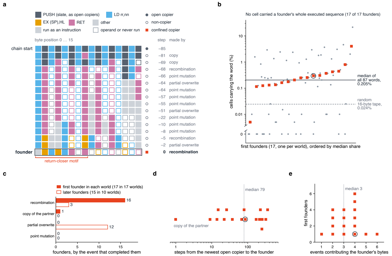
Extended Data Fig. 7 | The first self-confined copier of each world was completed by recombination, from parts circulating in non-copiers. a , The line of descent in world 31010 (the chain closest to the median, 14 records over 79 steps), from the newest open copier older than the founder (chain start) to the founder (boxed); each row is a record, with its step relative to the founder and the event that made it. Bytes are coloured by value (PUSH slate, the open-copier colour); a filled byte is an instruction start in at least half of 64 encounters with random partners, an outlined byte only an operand or never run; markers give each tape's class against the same partners. The half of the founder that runs is the return-closer motif. b , For each of the 17 first founders, the share of the 20,000 cells carrying each two-byte word that begins at one of its instruction starts (grey; 87 words) in the last soup snapshot before the founder; squares, each founder's median; ring, the world in a ; solid line, the median of all words; dashed, the expectation for a random 16-byte tape. Words carried by no cell (15 of 87) are drawn below the break; no cell carried any founder's whole executed sequence. c , The event that completed each founder: first founders (filled; one in each of 17 worlds) and later founders in the same worlds (open; 15 in 10 worlds). d , Steps from the newest open copier to each first founder. e , Distinct events that set the founder's bytes. Recombination: the new tape keeps less than 75% of its own bytes and is not a \geq 75\% copy of its partner; partial overwrite: it keeps at least 75%; copy of the partner: it becomes a \geq 75\% copy of its partner; point mutation: the simulator's mutation operator. Exploratory: the chain start, the separation of first from later founders and the word measure were defined after the recorded lines were inspected (Methods).
