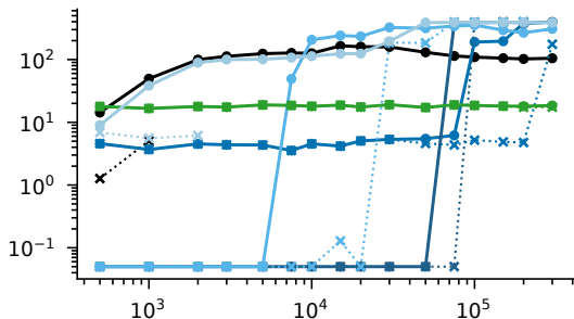
step programs destroyed per 1,000 interactions
