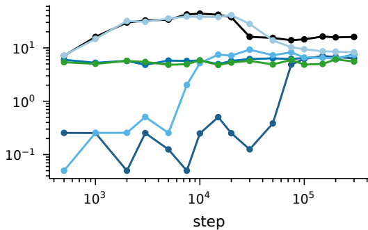
step programs destroyed per 1,000 interactions
