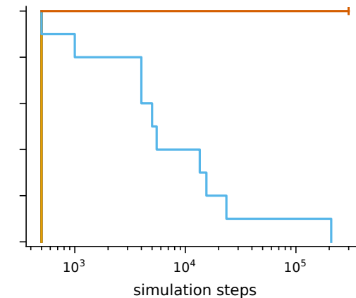
Time to first replicator, L = 100 bytes (Kaplan-Meier; ticks = censored at the run's last step) 128 steps · mutation 1/2^4
