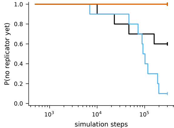
Time to first replicator, L = 9 bytes (Kaplan-Meier; ticks = censored at the run's last step) 128 steps · mutation 1/2^4
