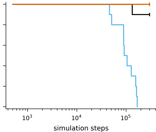
Time to first replicator, L = 9 bytes (Kaplan-Meier; ticks = censored at the run's last step) 128 steps · mutation 1/2^4
