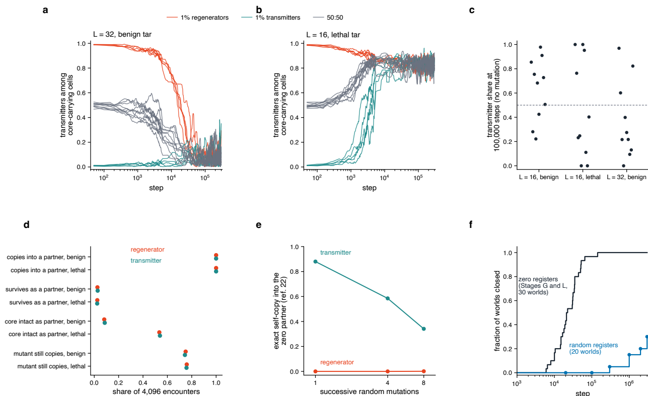
Extended Data Fig. 10 | The copy-offset switch and closure without supplied registers. a, b , A regenerator R and a transmitter T with the same core, XX\ 5e\ ed\ b0 , differing only in the offset byte and in what follows the core ( L = 32 : R = 04\ 5e\ ed\ b0 \times 8 , T = a0\ 5e\ ed\ b0 + 28 random bytes; L = 16 : R = 44\ 5e\ ed\ b0 \times 4 , T = b0\ 5e\ ed\ b0 + 12 random bytes, drawn for every cell), with the standard mutation: transmitters among the cells carrying the core against step, from 1% regenerators (vermillion), 1% transmitters (teal) or a 50:50 mixture (grey); one line per world (five, five and ten); samples with fewer than 1,000 core-carrying cells are omitted, and after step 5,000 each line is a running median of nine samples. At L = 32 with benign tar every start converges to a low transmitter share, at L = 16 with lethal tar to a high one; under lethal tar the core was later lost in 7 of 20 worlds (1 of 5 from 1% regenerators, 3 of 5 from 1% transmitters, 3 of 10 mixtures). At L = 16 with benign tar and mutation the core fell below 1,000 cells in all 20 worlds, and that condition is not shown. c , Without mutation the share drifts: transmitter share at 100,000 steps in each of ten 50:50 worlds per condition (dashed, the start). d , Encounter components of the pristine pair at L = 16 (4,096 encounters each; partners and executors drawn from the final soups of the mixed worlds of each tar, under benign tar soups in which the core had collapsed): exact copy into a partner, exact survival as the partner of a soup executor, core bytes 1–3 intact as a partner, and exact copying by a random single mutant. e , Post hoc, ref. 22’s robustness criterion for the L = 32 pair (exact self-copy into the all-zero partner, 512 instructions, after k successive random mutations; 1,000 trials; median over 20 transmitter tails): the transmitter scores high because it keeps mutations, the regenerator near zero because it erases them. f , Closure at L = 16 with zero registers (black: fraction of the 30 worlds of Stages G and L whose first closed common tape has appeared) and with every register drawn at random before each encounter (blue: fraction of 20 worlds in which most heritable cells among 64 random cells are confined, at the recorded snapshots); the two criteria differ, and the second is the stricter.
