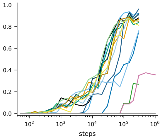
fraction of random cells heritable (gen2 \geq 0.3 )
