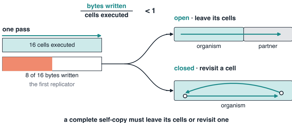
Fig. 6 | Closure requires a cycle. Theorem 2 as a diagram. A program that writes fewer bytes than the cells it executes cannot copy itself in one pass: the first replicator (L = 16) executes its 16 cells and has written 8 of the 16 bytes a copy needs (executor trace), so copying requires more execution, which can only continue outside its cells (open) or revisit one of them (closed, a cycle). Proofs, the closure-window model and the lemma on information inflow are in the Supplementary Information.
