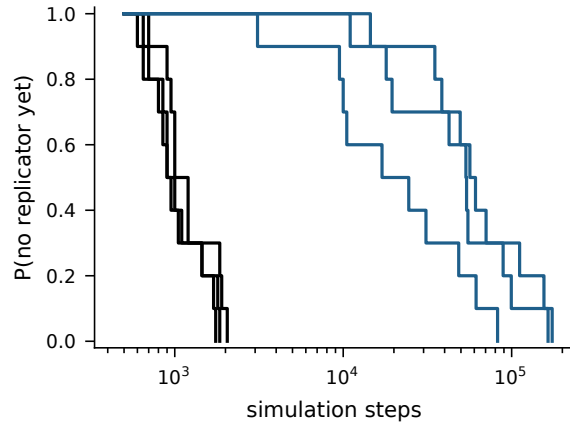
Time to first replicator, L = 25 bytes (Kaplan-Meier; ticks = censored at the run's last step)
