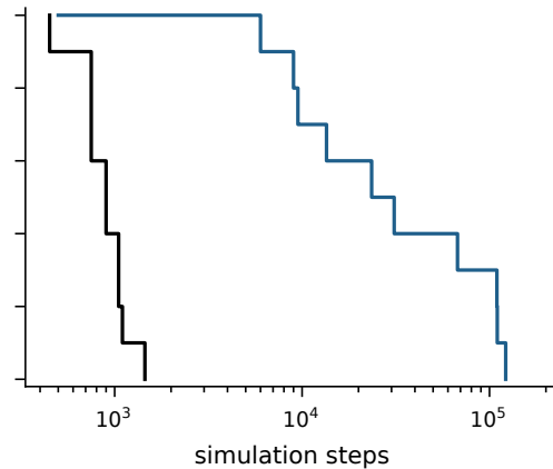
Time to first replicator, L = 25 bytes (Kaplan-Meier; ticks = censored at the run's last step)
