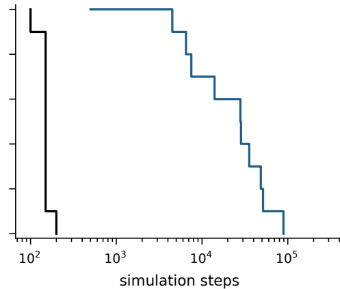
Time to first replicator, L = 81 bytes (Kaplan-Meier; ticks = censored at the run's last step)
