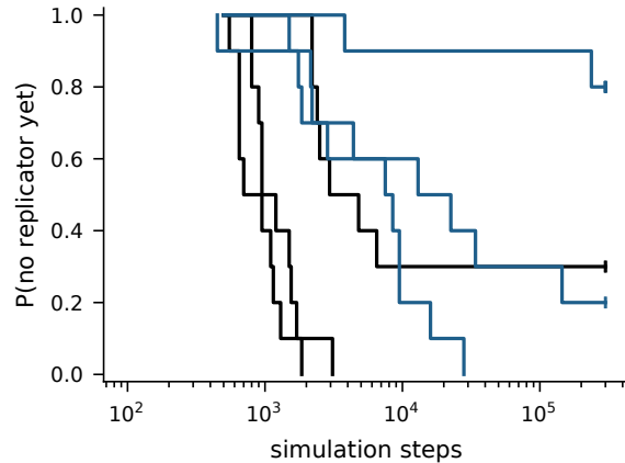
Time to first replicator, L = 81 bytes (Kaplan-Meier; ticks = censored at the run's last step)
