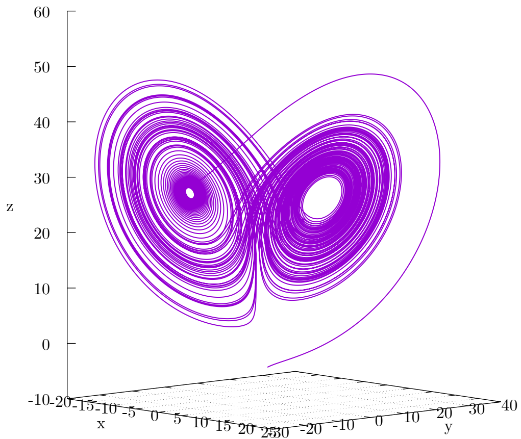
Lorenz Butterfly for initial condition (1, 2, -4)
