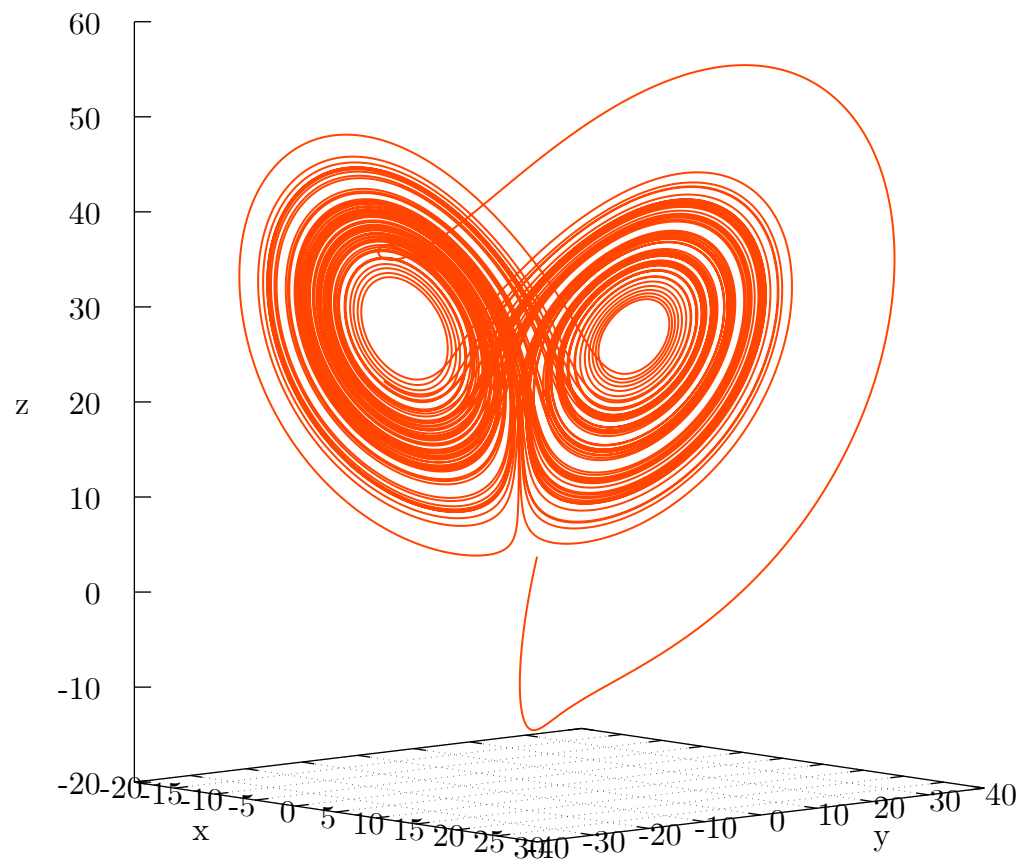
Lorenz Butterfly for initial condition (30, -40, 10)
