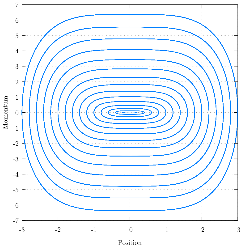
Phase Portrait (Pure Quartic Oscillator)
