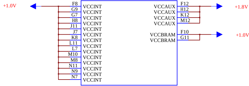
U1-H XC7A15TCSG324
