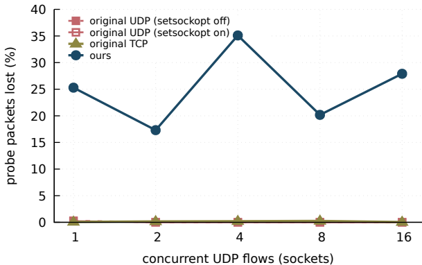
MTU 1500: probe-flow loss
