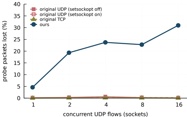
MTU 9000: probe-flow loss
