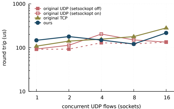
MTU 9000: probe round trip (p50)
