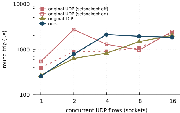
MTU 1500: probe round trip (p99)
