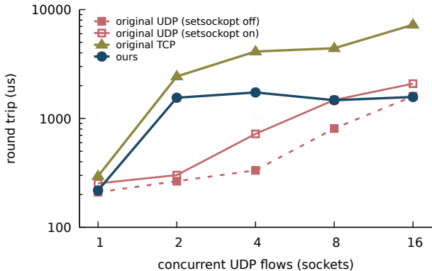
MTU 9000: probe round trip (p99)
