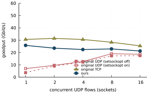
MTU 1500: throughput
