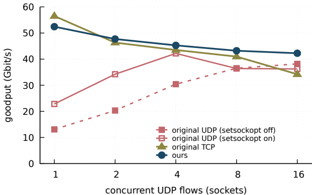
MTU 9000: throughput
